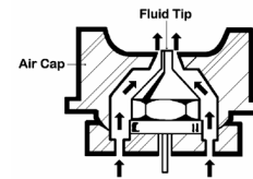
Figure 2 - Siphon Feed Air Cap
