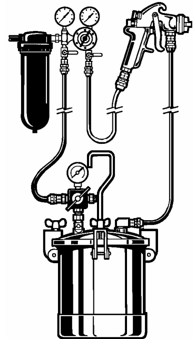
Figure 16 - Pressure Feed System Components
